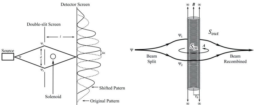
Figure 2. The AB effect. A beam of electrons \Psi is split in a region S_{out} , made to encircle a solenoid (that generates a magnetic field inside the region S_{in} ), and then to recombine on a detector screen. The original interference pattern is shifted by an amount \Delta x .
