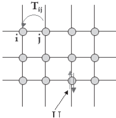
Figure 8. Schematic representation of the processes modeled by the Hubbard Hamiltonian: U is the Coulomb repulsion experienced by two electrons (of opposite spin) occupying the same site in a crystal lattice; T_{ij} are the hopping integrals that apply to the movement of an electron from one lattice site, j , to another, i .
