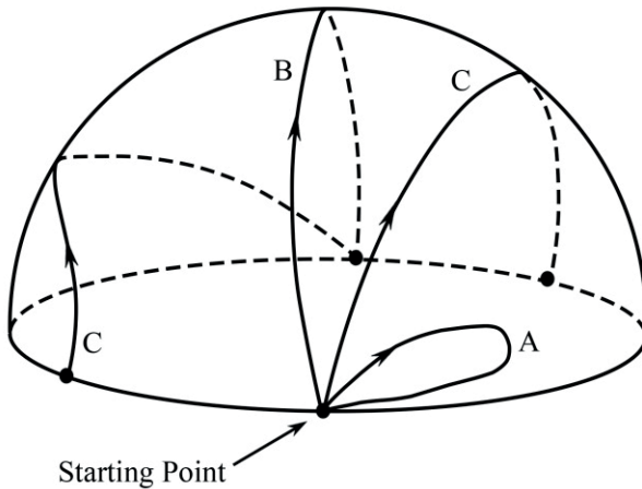
Figure 5. The real projective space in two dimensions RP_2 , represented by the northern hemisphere with opposite points on the equator identified.
